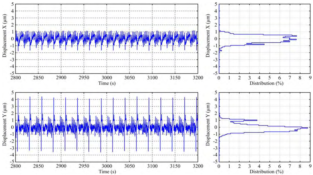
Figure 11: Measured displacements and histograms in x and y direction.
